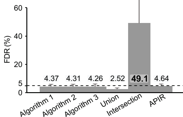
Figure 3 Simulation studies showing that neither intersection nor union of discovery sets (with controlled FDR) controls FDR
