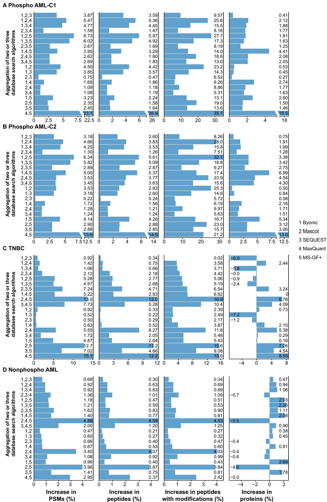
Figure 5 Power improvement of APIR over individual database search algorithms at the FDR threshold q = 5\% The percentage increases in PSMs (first column), the percentage increases in peptides (second column), the percentage increases in peptides with modifications (third column), and the percentage increases in true proteins (fourth column) of APIR after aggregating two or three database search algorithms out of the five (Byonic, Mascot, SEQUEST, MaxQuant, and MS-GF+) at the FDR threshold q = 5\% on the phospho AML-C1 dataset (A), the phospho AML-C2 dataset (B), the TNBC dataset (C), and the nonphospho AML dataset (D). The percentage increase in PSMs/peptides/peptides with
